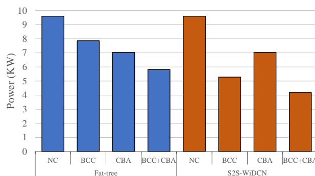
Figure 12. Power consumption comparison between normal condition, BCC, CBA and combination of BCC and CBA.
